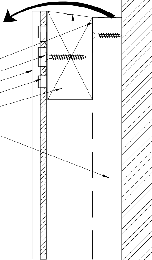
Section on Profile 1:2
