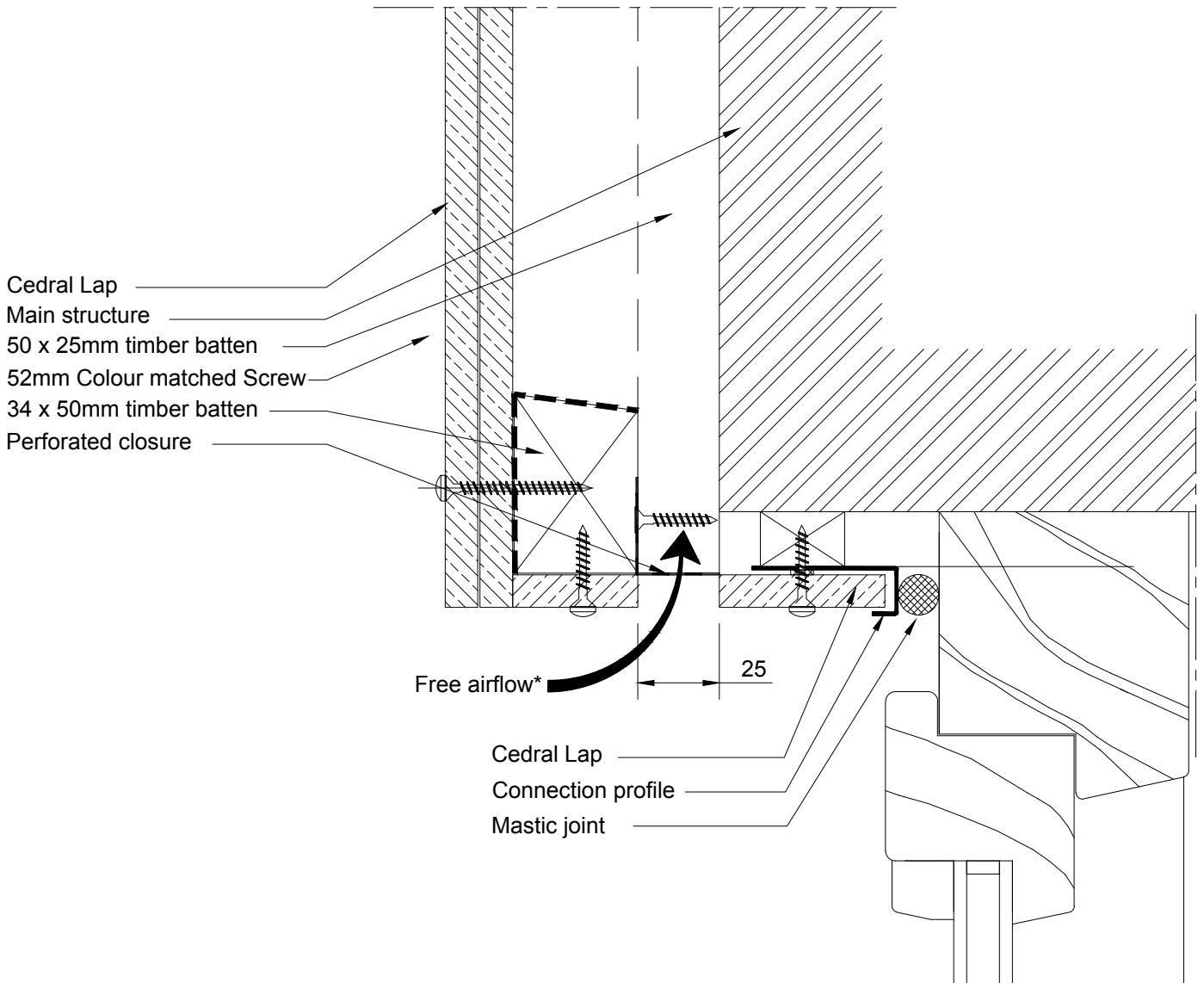
Section on Profile 1:2
